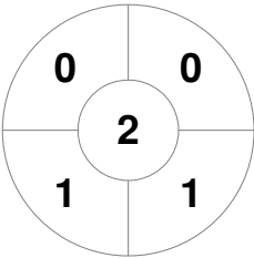
VIPERS 2
