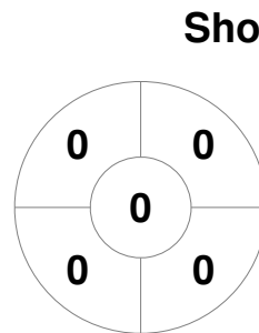
BUND1
